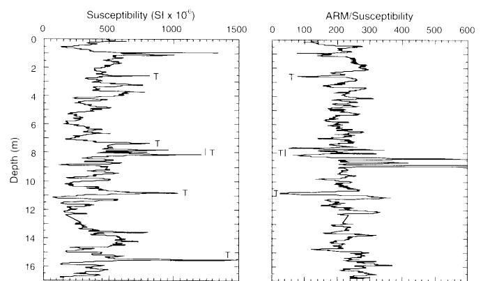
Figure 3. Magnetic susceptibility and ARM/susceptibility records for Hole 883D. Each T indicates a prominent tephra layer.
