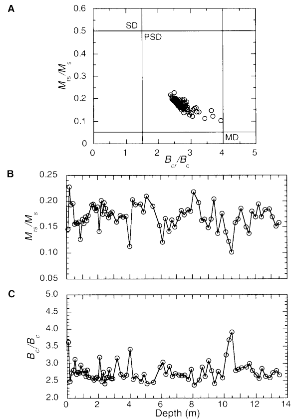
Figure 8. Grain-size variation for Hole 884D as indicated by high-field magnetic hysteresis data. A. Bivariate plot of M_{rs}/M_s vs. B_{cr}/B_c . Fields are shown for SD, PSD, and MD grains (after Day et al., 1977). B. M_{rs}/M_s vs. depth. C. B_{cr}/B_c vs. depth.
