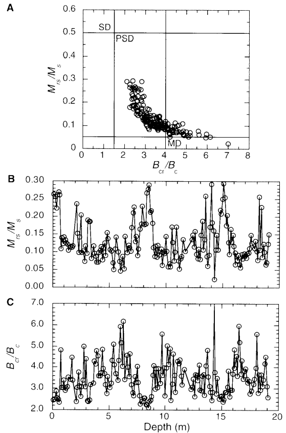
Figure 13. Grain-size variation for Hole 887B as indicated by high-field magnetic hysteresis data. A. Bivariate plot of M_{rs}/M_s vs. B_{ct}/B_c . Fields are shown for SD, PSD, and MD grains (after Day et al., 1977). B. M_{rs}/M_s vs. depth. C. B_{ct}/B_c vs. depth.
