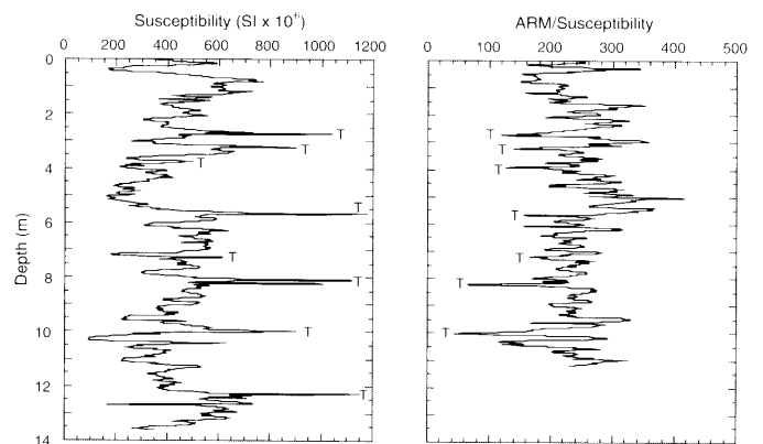
Figure 4. Magnetic susceptibility and ARM/susceptibility records for Hole 884D. Each T indicates a prominent tephra layer.
