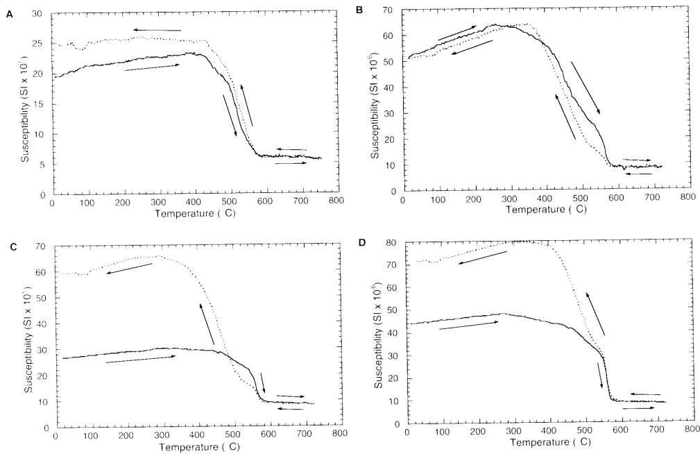
Figure 9. Temperature dependence of magnetic susceptibility for selected samples. A. Sample 145-883D-2H-2, 70 cm. B. Sample 145-884D-2H-3, 80 cm. C. Sample 145-887B-2H-5, 70 cm. D. Sample 145-887B-2H-6, 70 cm. Solid line indicates heating curve; dashed line indicates cooling curve. Major drop in susceptibility above 550°C indicates a magnetic mineral assemblage that is dominated by magnetite. Note difference in susceptibility scale for Figure 9A.
